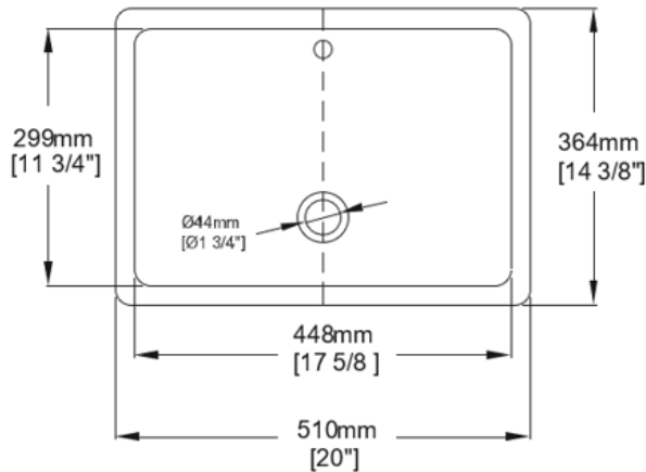
SINK DIMENSIONS • Diagrams not to scale. • All measurements ±1/4".
